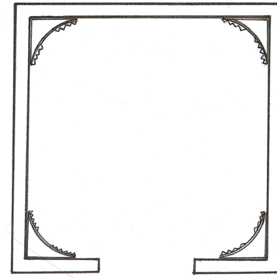
○ PLAN (OPTION B) 1/2" = 1' - 0"
