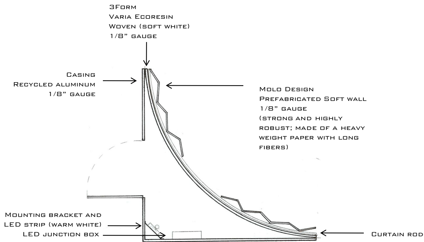
○ PLAN CUT 3" = 1' - 0"
