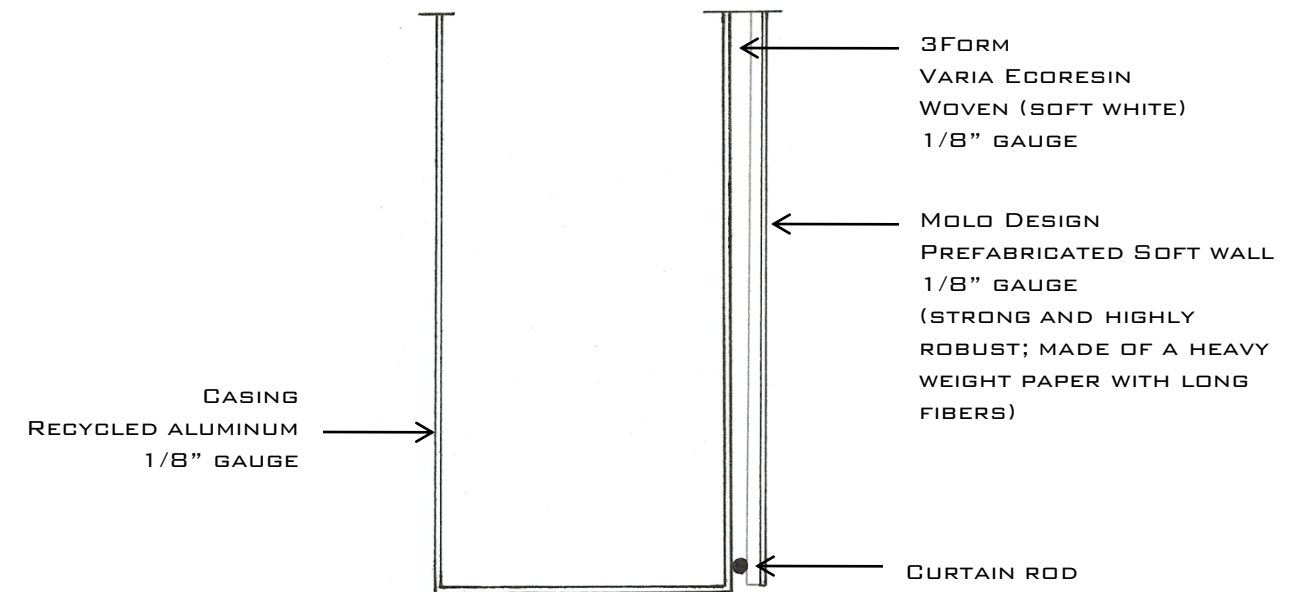
○ SECTION 3" = 1' - 0"
