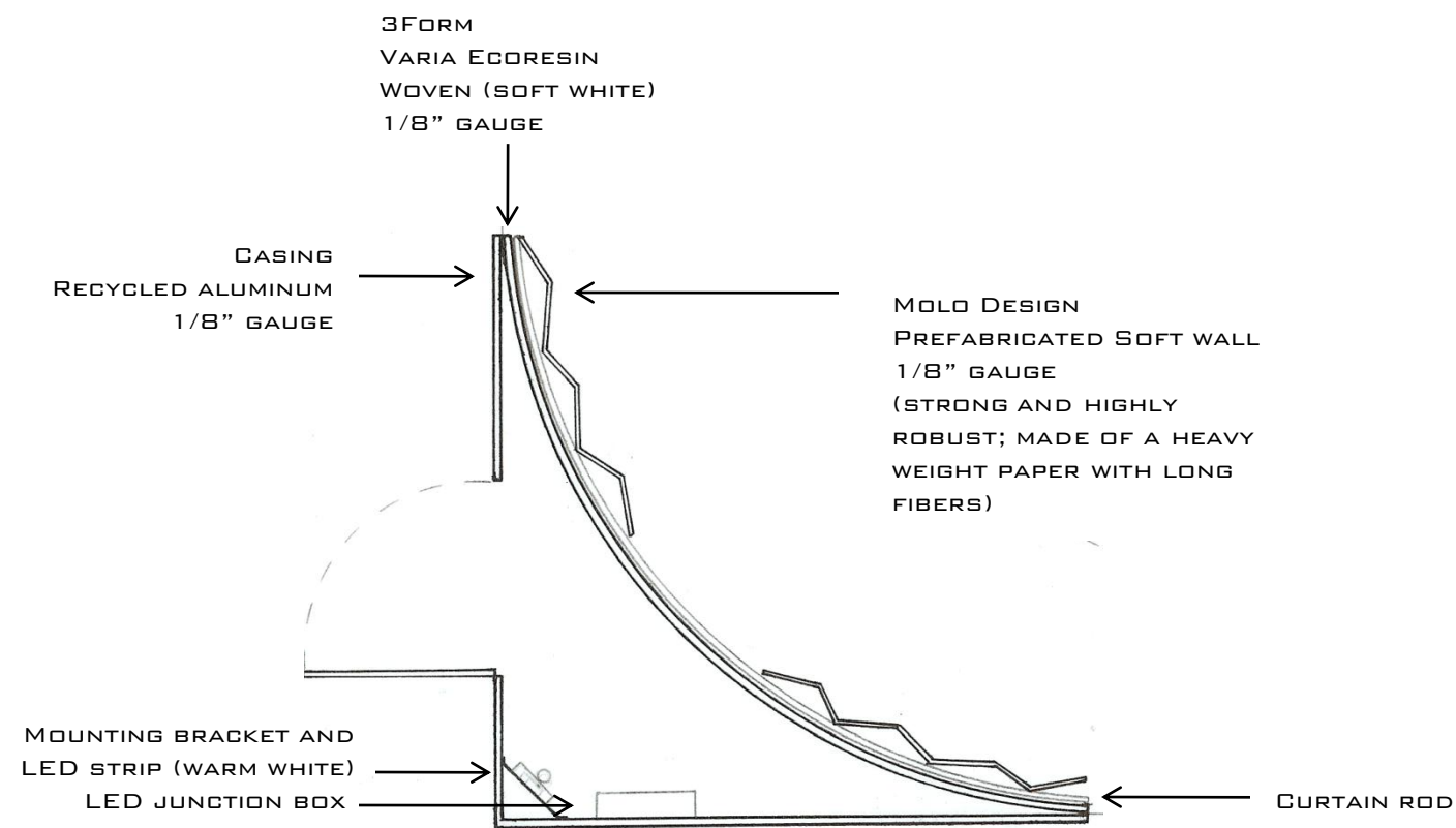
○ PLAN CUT 3" = 1' - 0"
