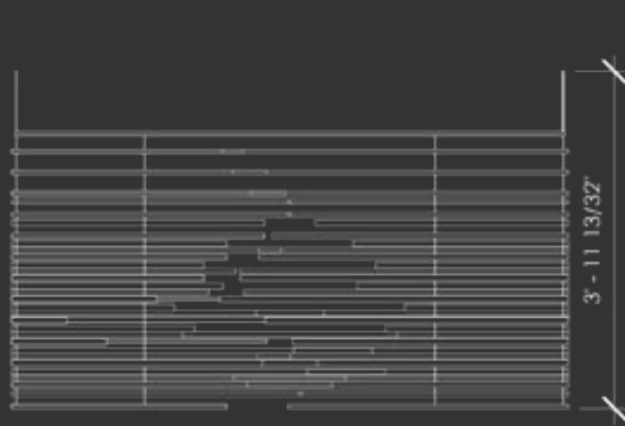
HORIZON PENDANT 6.5' MODULE front elevation scale 1/2" = 1'0"
